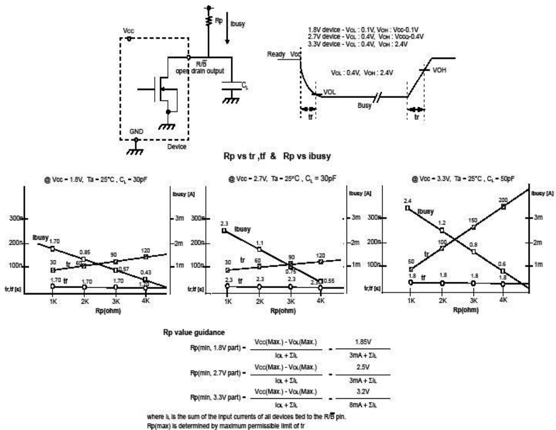
Figure 33 : Ready/Busy Pin electrical application
