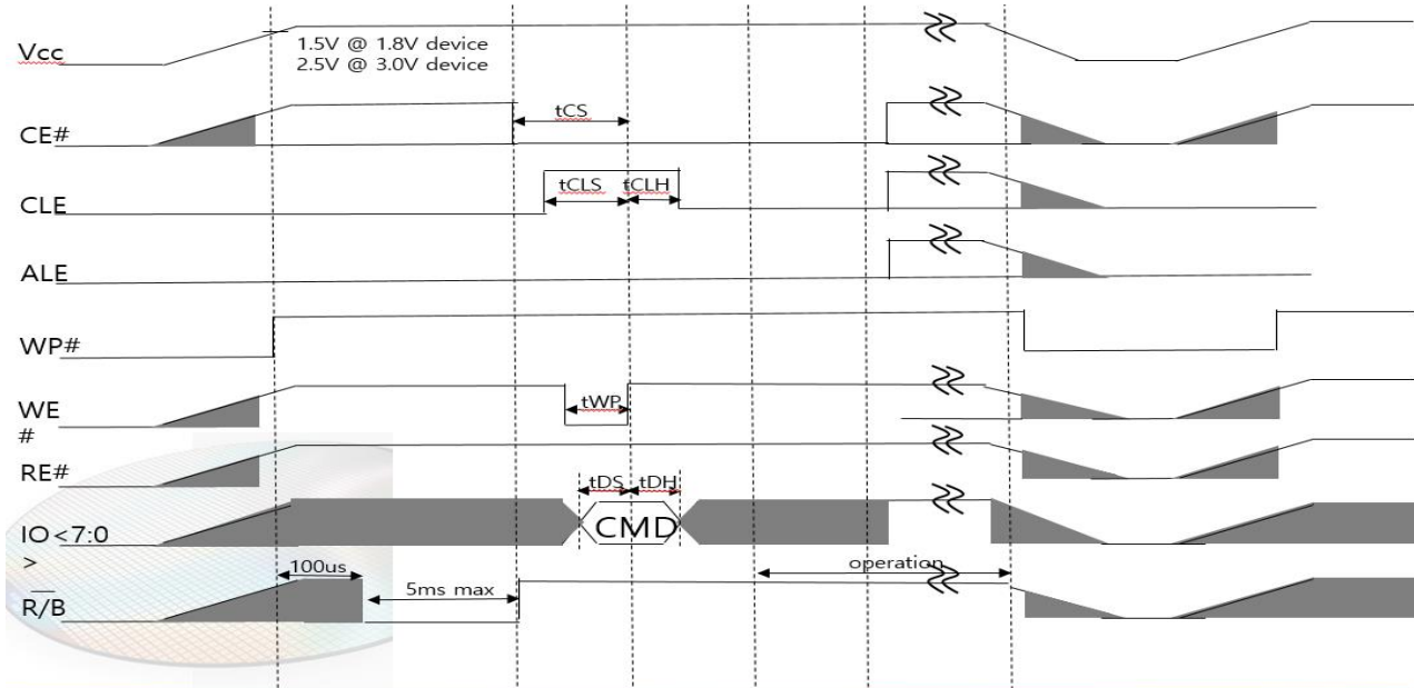
Figure 32 : power up time sequence
