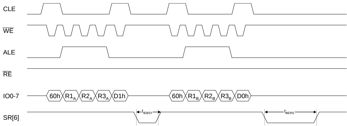
Figure 25: Multiple plane block erase (ONFI 1.0 protocol)
