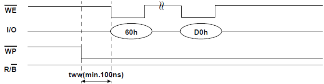
Figure 31 : tWW in Erase Operation
